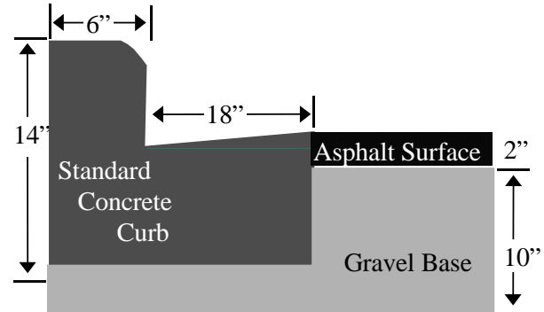
Standard Curb
