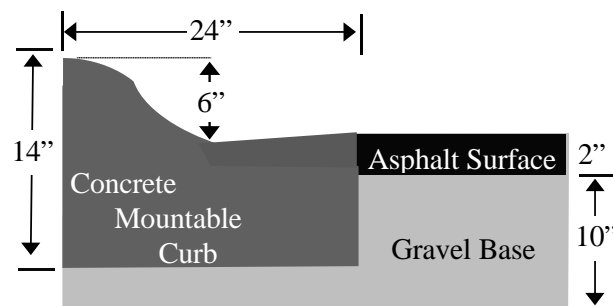
Mountable Curb
